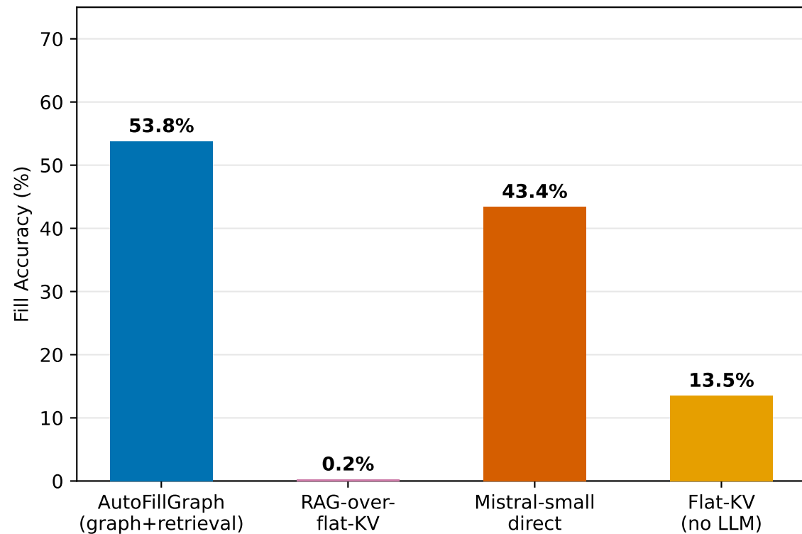
FUNSD Fill Accuracy (178 docs)
