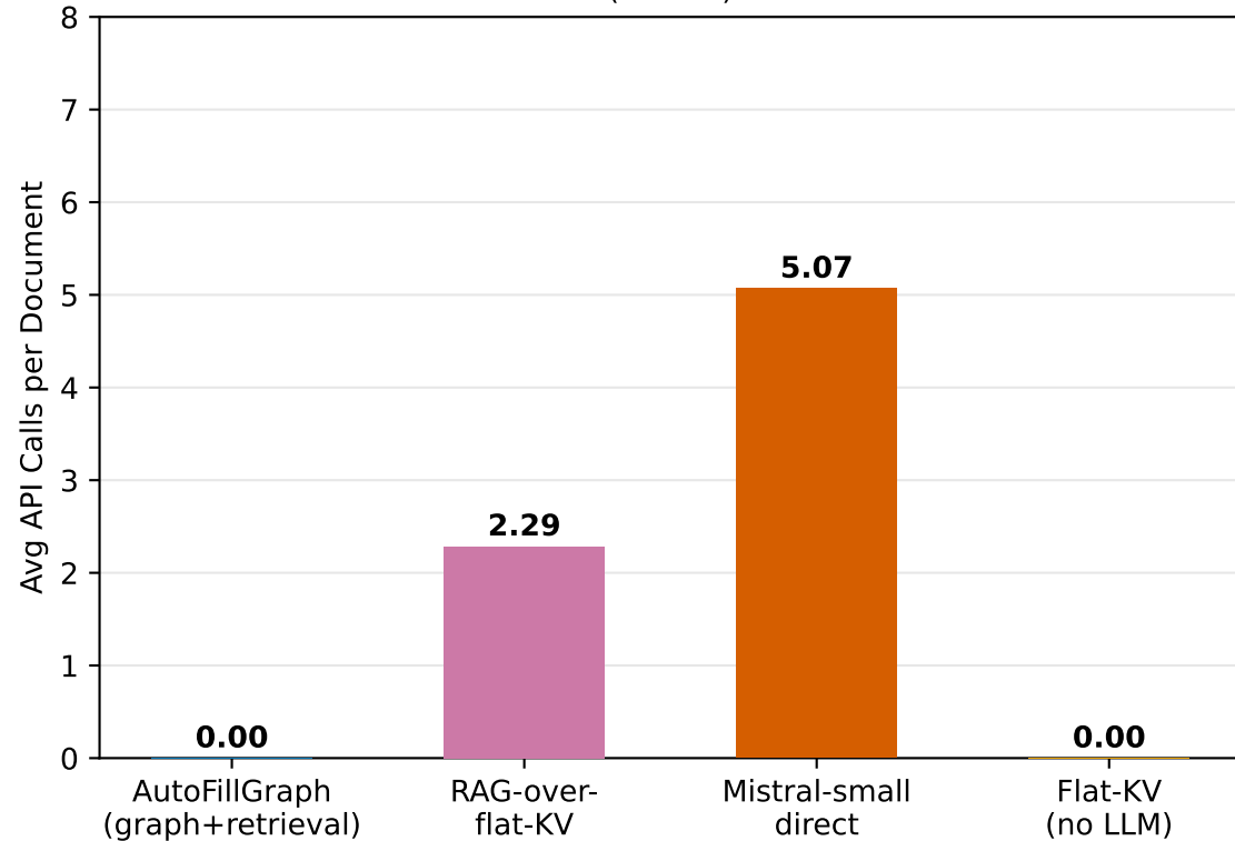
API Call Efficiency (FUNSD)
